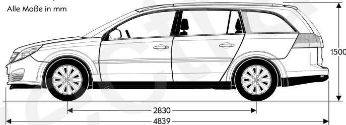
Vectra, Caravan
